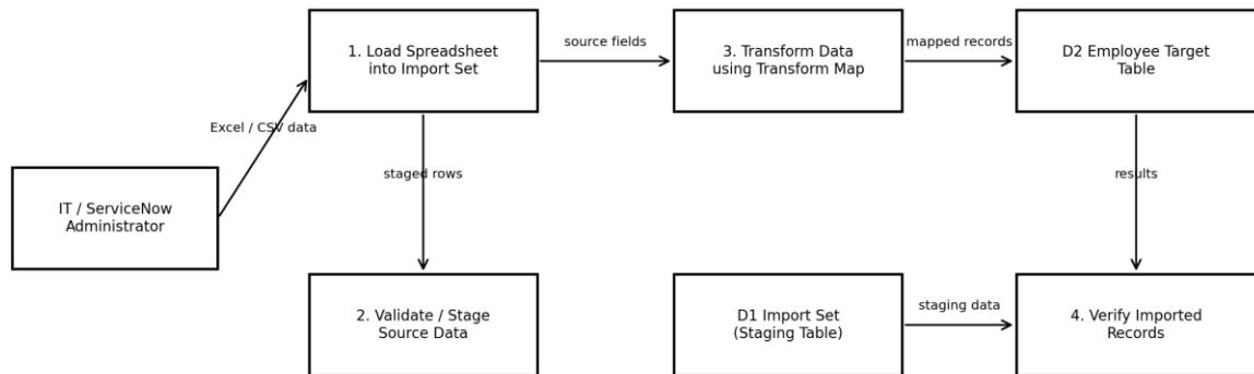
DFD Level 0 - Spreadsheet Import using Import Sets & Transform Maps
